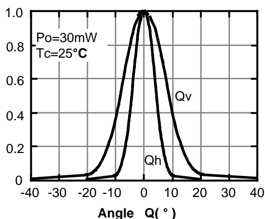
Beam divergence
